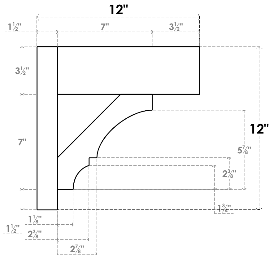
SIDE PROFILE
